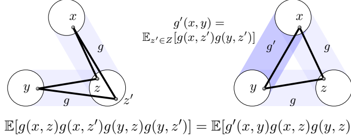
FIGURE 4. The densification step in the proof of the relative triangle counting lemma.
